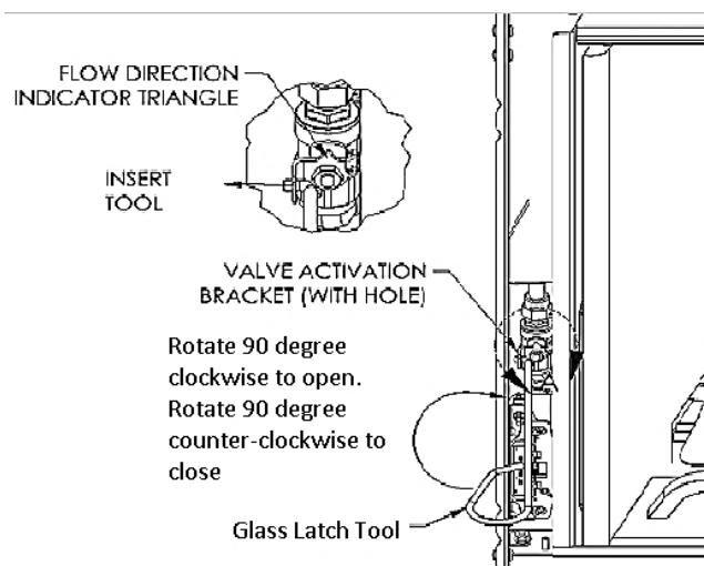
EMERGENCY GAS SHUTOFF
